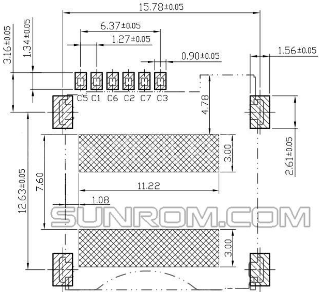
RECOMMENDED PCB PATTERN LAYOUT(TOP VIEW)
